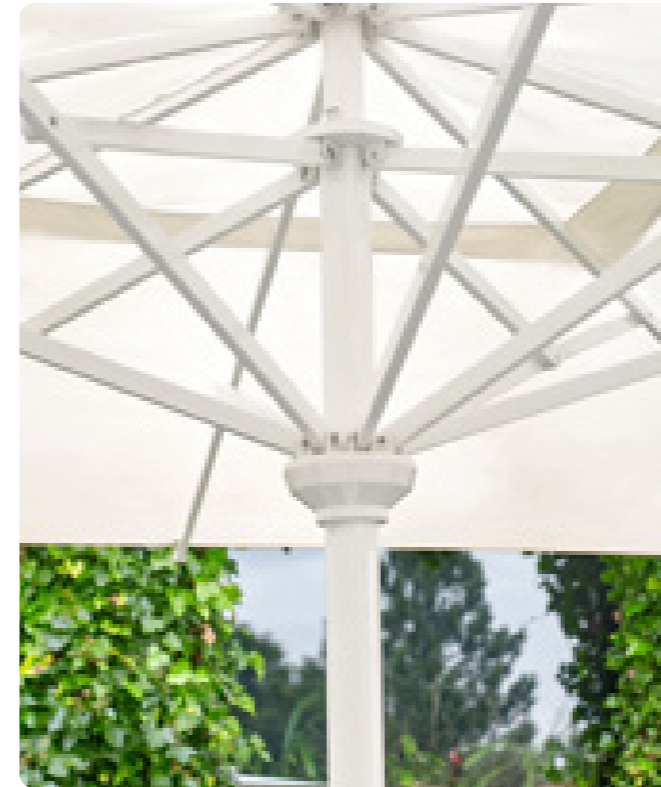
Exchangeable ribs.
