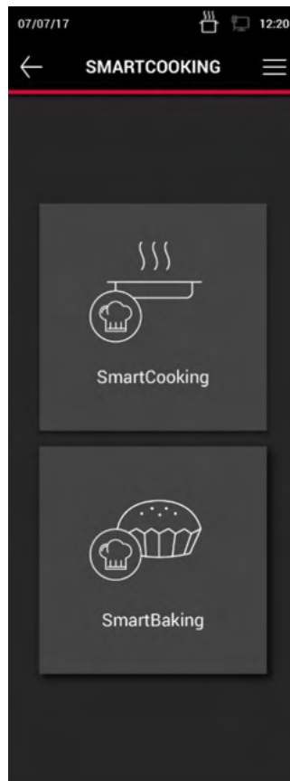
Figura 18. Pantalla SmartCooking
