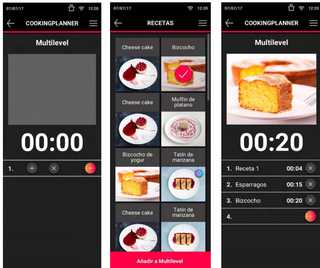
Figura 23. Pantallas CookingPlanner
